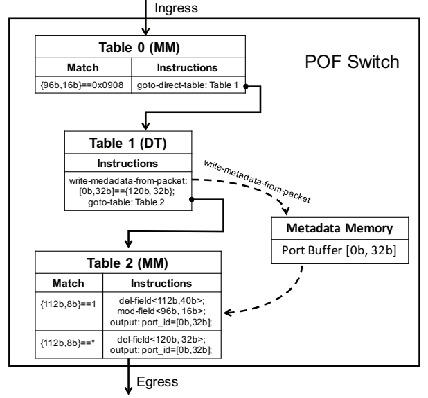
Fig. 6. Procedure used to process the flow tables in core switches for source routing.
